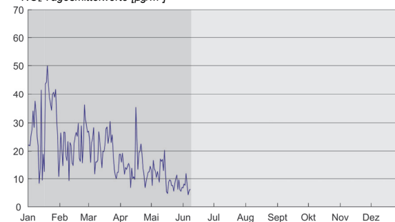
PM10 Tagesmittelwerte [ \mu\text{g}/\text{m}^3 ]
